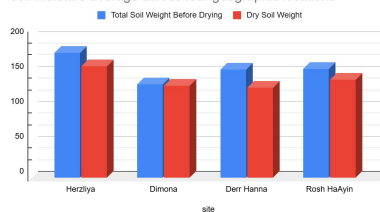
soil moisture average across four geographic locations
