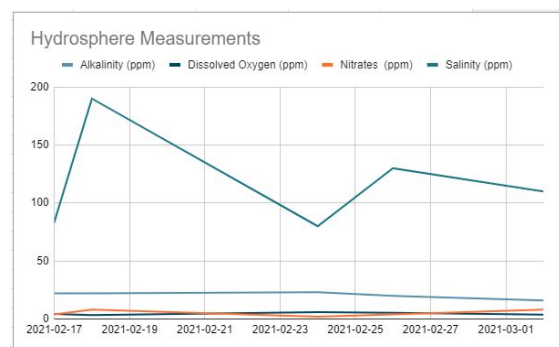
Graph 1. Hydrosphere Measurements
