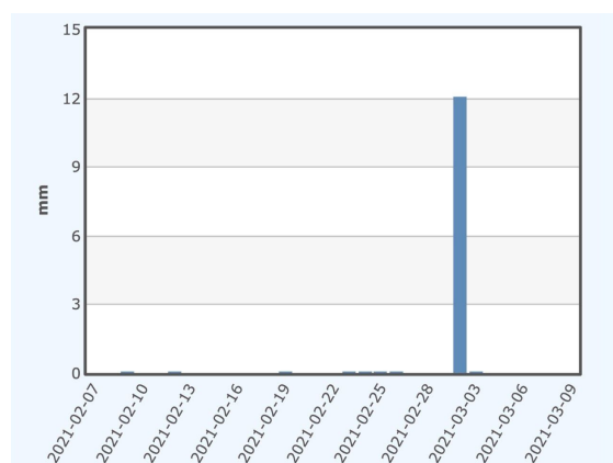
Graph 2. Precipitations
