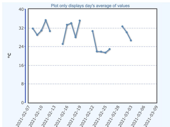
Graph 4. Temperature
