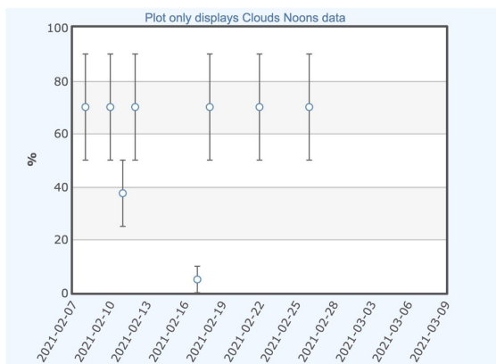
Graph 5. Clouds
