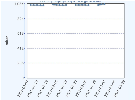
Graph 3. Barometric Pressures
