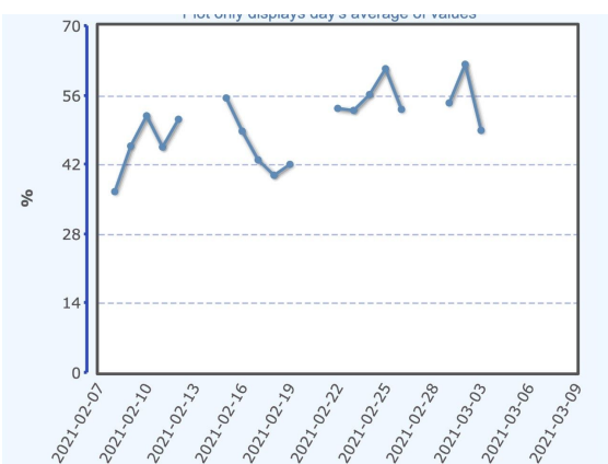
Graph 6. Relative Humidities
