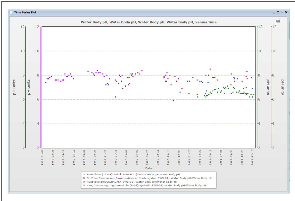
Figure HY-pH-3: Temporal pH Data for Certain Scandinavian GLOBE Schools
