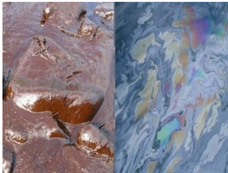
Figure 2. Persistent oil (left) and non-persistent oil (right).
