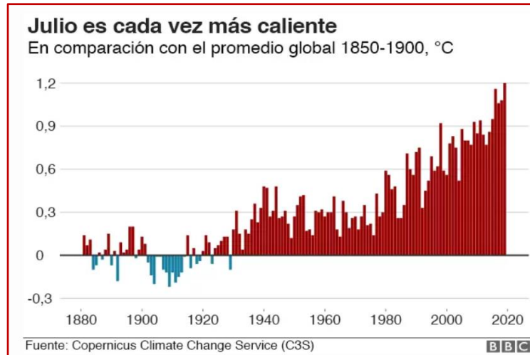
Fig. 4: Average temperature increase for the month from 1880 to 2020
