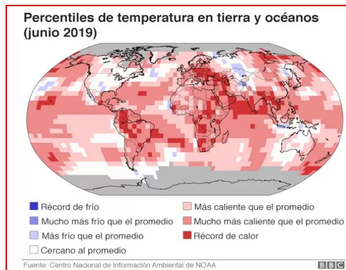
Fig. 3: Temperature in 2019. Source: NOAA.
