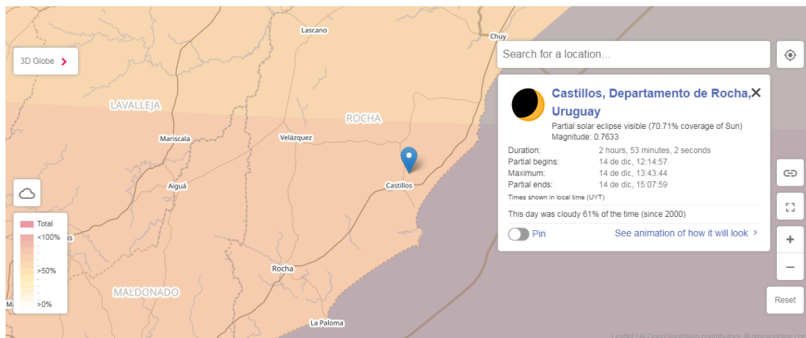
Fig. 6: Visualization of how an eclipse was observed in Castillos city, Rocha, Uruguay.
