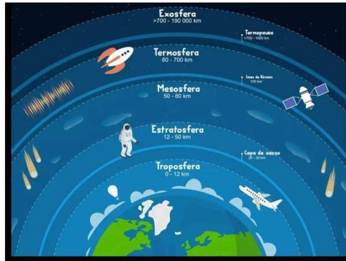
Fig. 3: Layers of the atmosphere Source: GeologiaWeb
