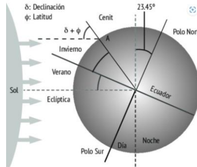
Fig. 1: Solar declination. This figure shows why the Equator receives the same amount of energy and gets warmer all year round, while the Poles only receive a considerable amount of energy in the summer. Source: (Cervantes, 2017)
