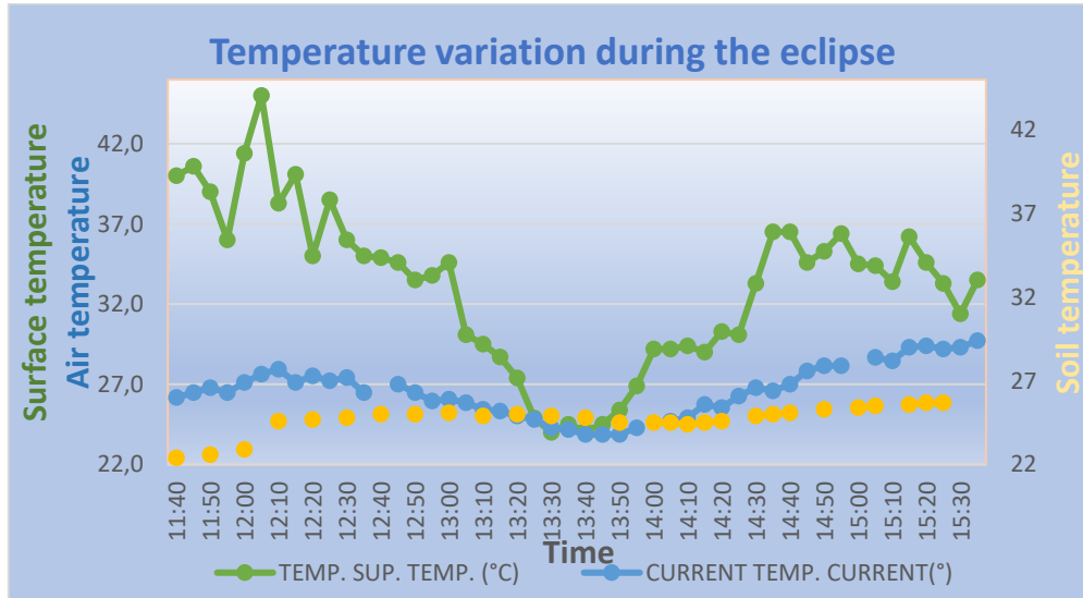
Fig. 3: Relationship of the variables air, surface and soil temperature during the December 14, 2020 eclipse. Source: Andrea Ventoso
